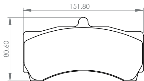
DP006- 54mm PAD TRACK
