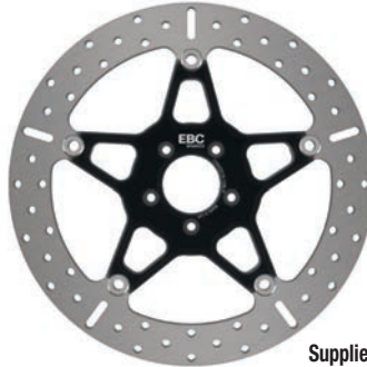
OSMD518-14BLK Fits EBC Pads: 400, 409, 457 BRK701 SEE RIGHT Supplied with relocation bracket & hardware
