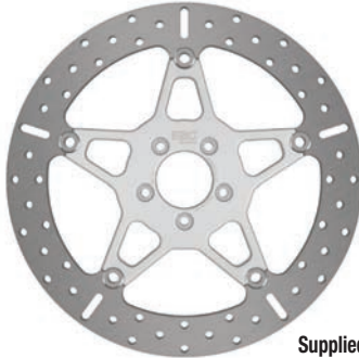
OSMD518-14 Fits EBC Pads: 400, 409, 457 BRK701 SEE RIGHT Supplied with relocation bracket & hardware
