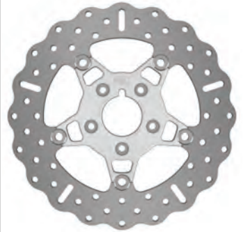
FSD011C Fits EBC Pads: 94, 216/3
